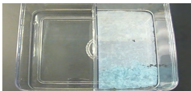
BRANDT REACTION
